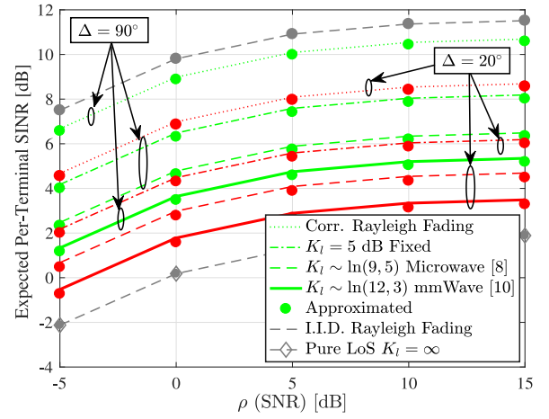
Fig. 1. Expected per-terminal SINR vs. \rho (SNR) with M = 32, L = 3 and \Delta = 20^\circ and 90^\circ .
