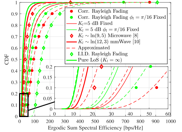
Fig. 2. Ergodic sum spectral efficiency CDF with M = 256, L = 32 at \rho = 10 dB and \Delta = 20^\circ .
